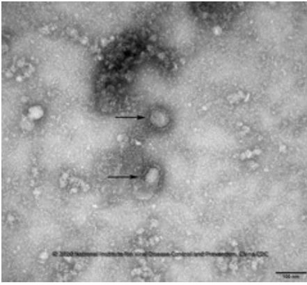
IVDC, China CDC: Wuhan coronavirus
